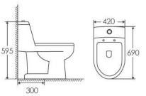
ET-2019 ONE-PIECE TOILET Siphonic 690×420×595mm S-trap 300mm
