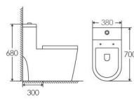
ET-2076 ONE-PIECE TOILET 2 Super Siphonic 700×380×680mm S-trap 300mm
