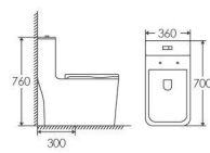
ET-2071 ONE-PIECE TOILET 4 Super Siphonic 700×360×760mm S-trap 300mm
