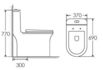
ET-2027 ONE-PIECE TOILET 2 Super Siphonic 690×370×770mm S-trap 300mm
