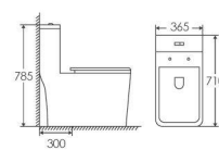
ET-2089 ONE-PIECE TOILET Siphonic 710×365×785mm S-trap 300mm
