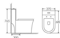
ET-2073C ONE-PIECE TOILET 4 Super Siphonic 680×370×765mm S-trap 300mm
