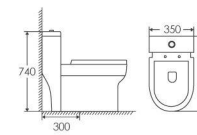
ET-2017 ONE-PIECE TOILET 2 Super Siphonic 650×350×740mm S-trap 300mm
