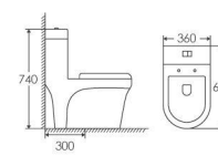
ET-2051 ONE-PIECE TOILET 2 Super Siphonic 640×360×740mm S-trap 300mm
