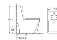
ET-2011 ONE-PIECE TOILET Siphonic/Washdown 680×370×790mm P-trap 180mm S-trap 250/300mm
