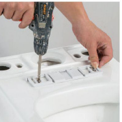
Install the screws from both sides
