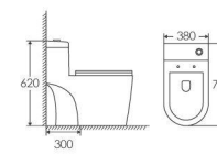
ET-2032 ONE-PIECE TOILET 2 Super Siphonic 710×380×620mm S-trap 300mm
