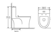
ET-2084C ONE-PIECE TOILET 4 Super Siphonic 700×385×705mm S-trap 300mm
