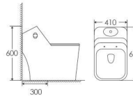
ET-2067 ONE-PIECE TOILET Siphonic 660×410×600mm S-trap 300mm
