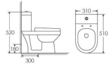
ET-001 ONE-PIECE TOILET Washdown 510×310×520mm P-trap 180mm S-trap 300mm
