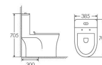
ET-2084 ONE-PIECE TOILET 4 Super Siphonic 700×385×705mm S-trap 300mm
