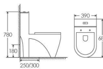
ET-2092 ONE-PIECE TOILET 2/4 Super Siphonic/Washdown 685×390×780mm P-trap 180mm S-trap 250/300mm
