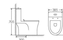
ET-2084B ONE-PIECE TOILET 4 Super Siphonic 700×385×705mm S-trap 300mm
