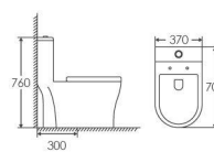
ET-2086 ONE-PIECE TOILET 2 Super Siphonic 700×370×760mm S-trap 300mm
