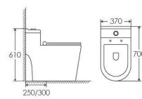
ET-2083 ONE-PIECE TOILET Siphonic 700×370×610mm S-trap 250/300mm
