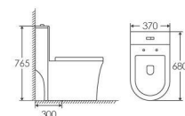
ET-2073B ONE-PIECE TOILET 4 Super Siphonic 680×370×765mm S-trap 300mm
