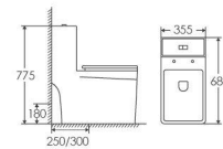
ET-2065 ONE-PIECE TOILET Siphonic/Washdown 680×355×775mm P-trap 180mm S-trap 250/300mm
