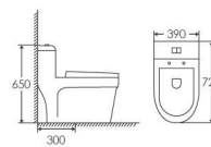
ET-2094 ONE-PIECE TOILET 2 Super Siphonic 720×390×650mm S-trap 300mm
