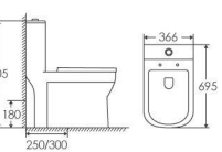
ET-2062 ONE-PIECE TOILET Siphonic/Washdown 695×366×805mm P-trap 180mm S-trap 250/300mm
