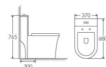
ET-2073 ONE-PIECE TOILET 4 Super Siphonic 680×370×765mm S-trap 300mm
