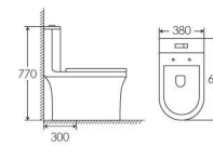
ET-2034 ONE-PIECE TOILET 4 Super Siphonic 680×380×770mm S-trap 300mm
